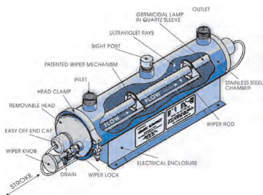
Ultraviolet light purifier
